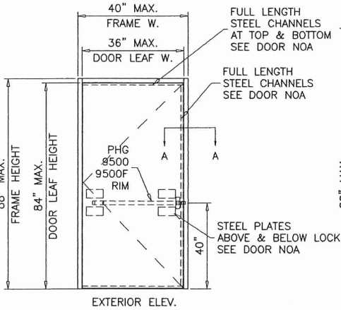
OUTSWING SINGLE STEEL DOOR UNDER SEPARATE APPROVAL
