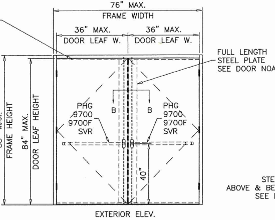
OUTSWING SINGLE OR DOUBLE STEEL DOOR UNDER SEPARATE APPROVAL
