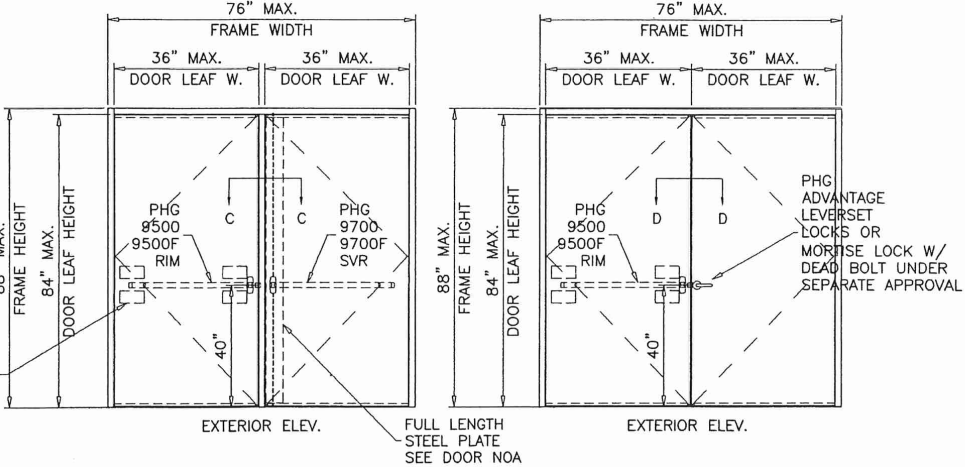
OUTSWING STEEL DOORS WITH INTERMEDIATE MULLION UNDER SEPARATE APPROVALS
