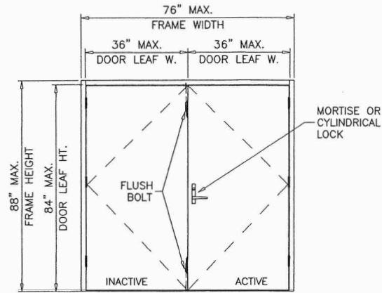
DOUBLE OUTSWING STEEL DOOR UNDER SEPARATE APPROVAL
