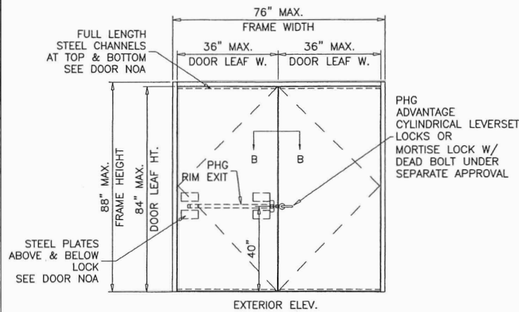
OUTSWING STEEL DOORS
