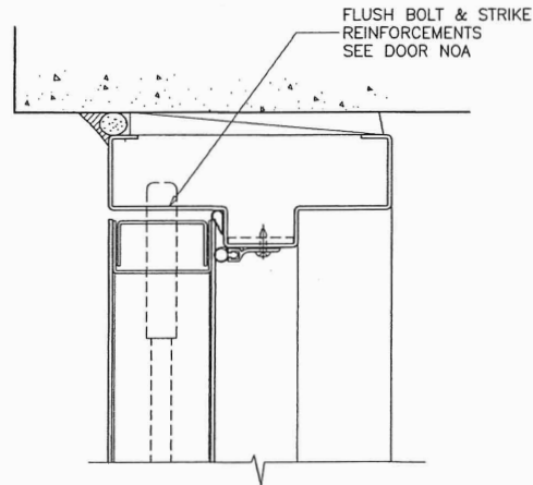
DOUBLE OUTSWING STEEL DOOR UNDER SEPARATE APPROVAL
