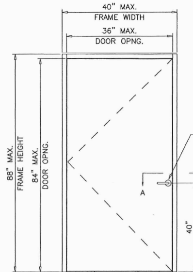
SINGLE OUTSWING STEEL DOOR
