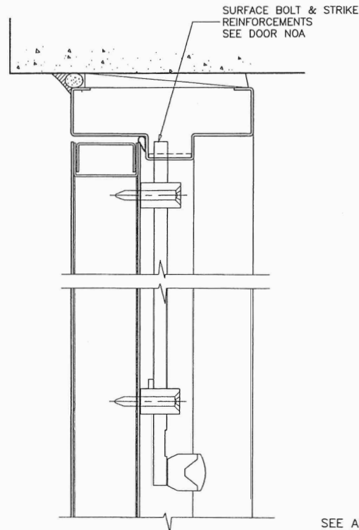
DOUBLE OUTSWING STEEL DOOR UNDER SEPARATE APPROVAL
