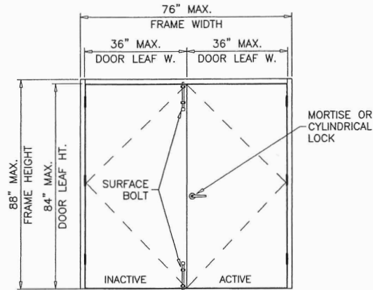
DOUBLE OUTSWING STEEL DOOR UNDER SEPARATE APPROVAL
