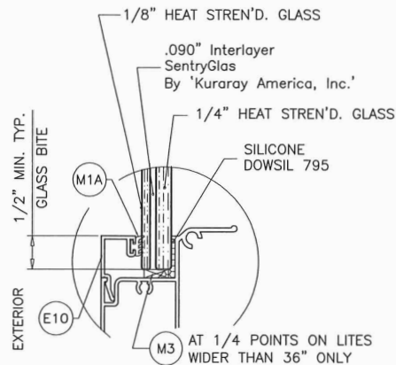
GLASS TYPE '2A' 7/16" OVERALL LAM. GLASS
