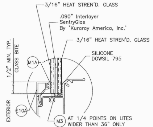
GLASS TYPE '3' 7/16" OVERALL LAM. GLASS
