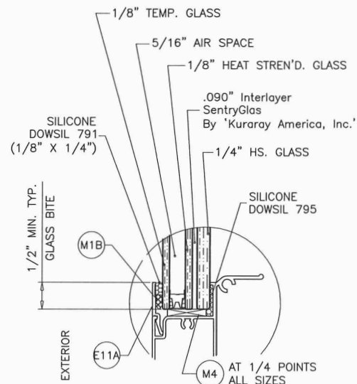
GLASS TYPE '2Ai' 7/8" OVERALL INSUL. LAM. GLASS
