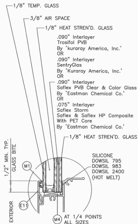
GLASS TYPE '1i' 7/8" OVERALL INSUL. LAM. GLASS
