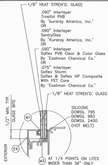
GLASS TYPE '1' 5/16" OVERALL LAM. GLASS
