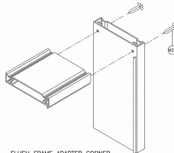
FLUSH FRAME ADAPTER CORNER
