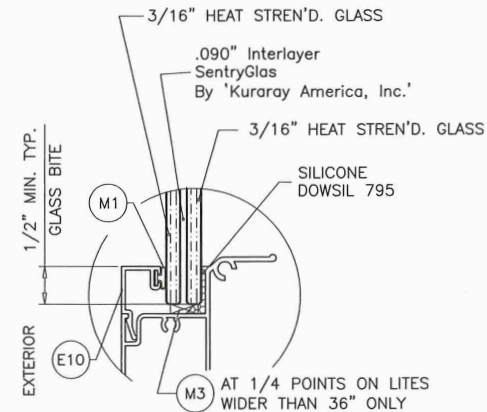
GLASS TYPE '3' 7/16" OVERALL LAM. GLASS
