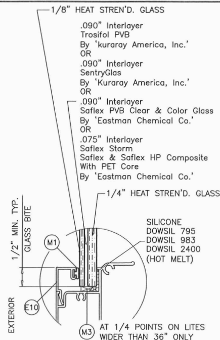
GLASS TYPE '2' 7/16" OVERALL LAM. GLASS
