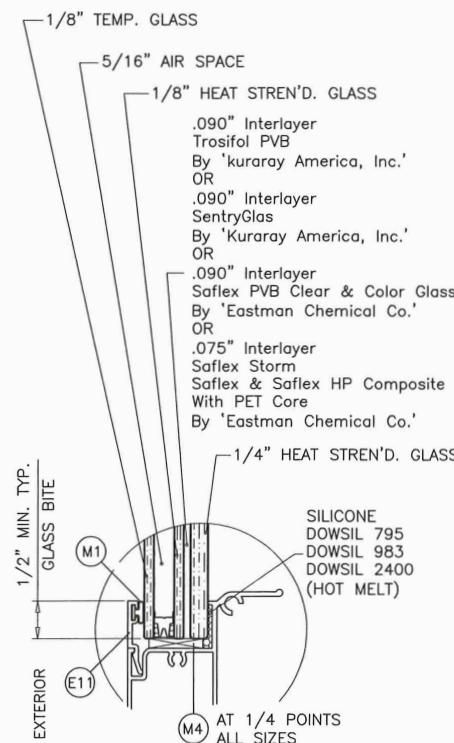
GLASS TYPE '2i' 7/8" OVERALL INSUL. LAM. GLASS
