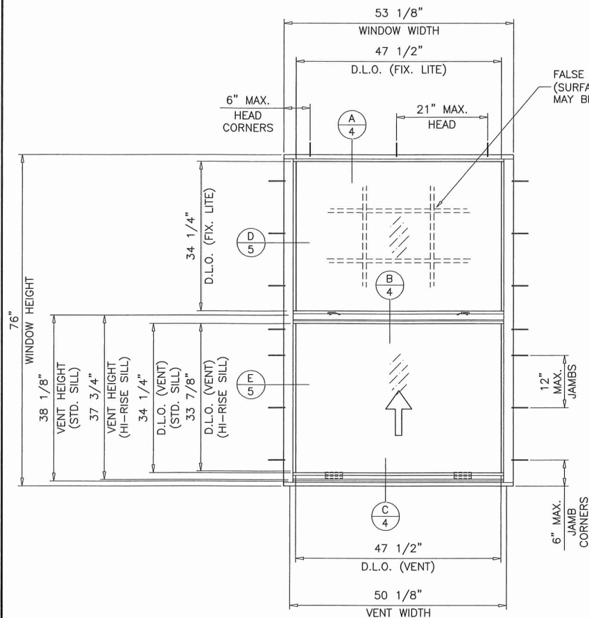
TYPICAL ELEVATION EQUAL LITES FLANGE FRAMES
