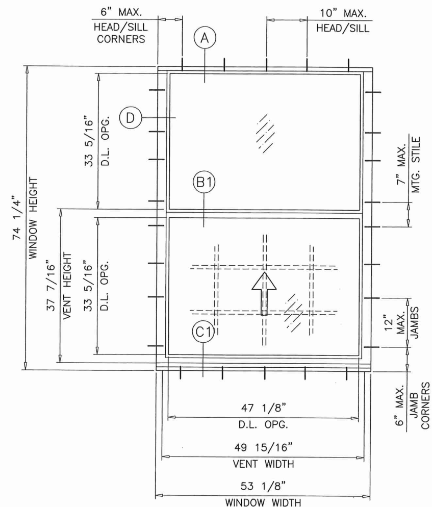
TYPICAL ELEVATION
