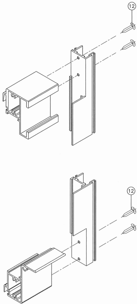
VENT TOP & BOTTOM CORNER
