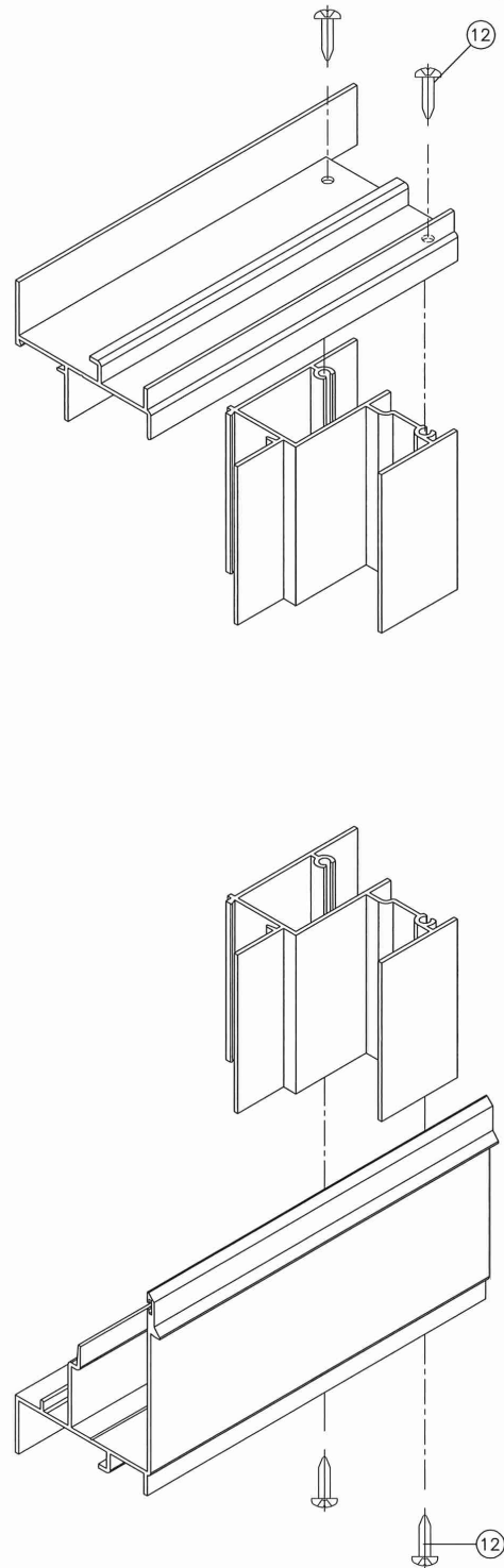
FRAME TOP & BOTTOM CORNERS
