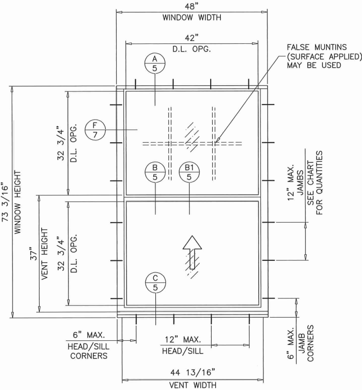
TYPICAL ELEVATION
