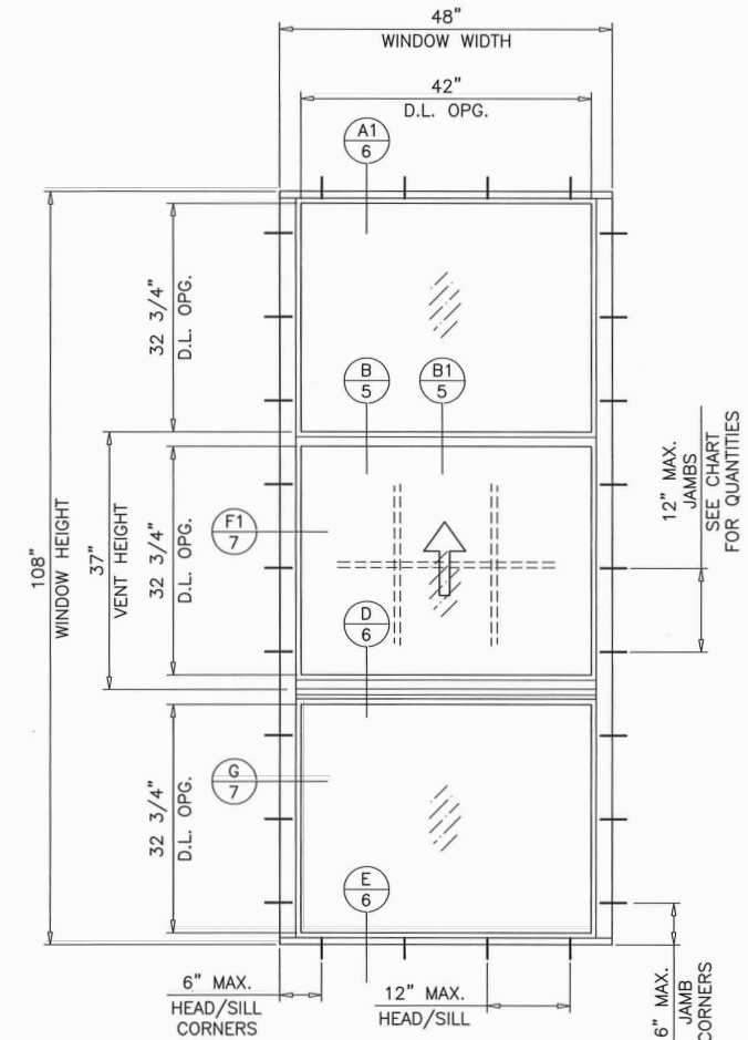
TYPICAL ELEVATION
