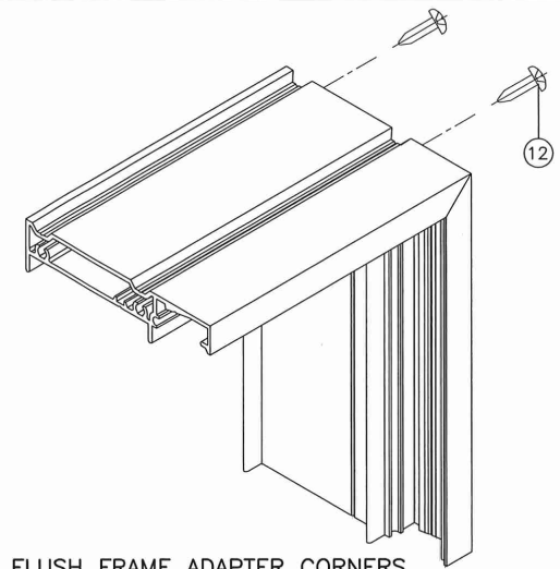
FLUSH FRAME ADAPTER CORNERS
