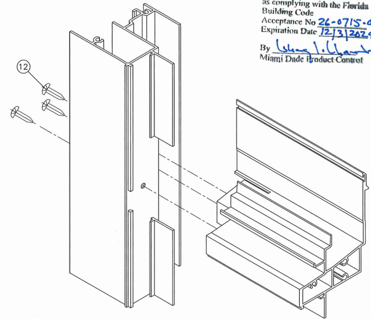
INTERMEDIATE SILL CORNER
