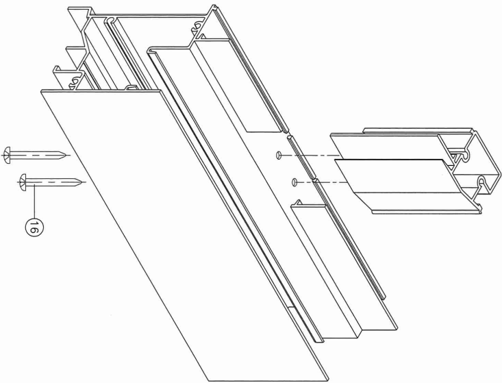
FIXED MTG. RAIL CORNER
