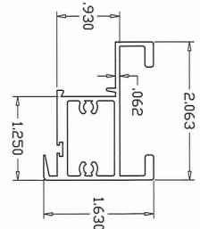
6A H.D. MEETING RAIL AT SWEEP LATCHES
