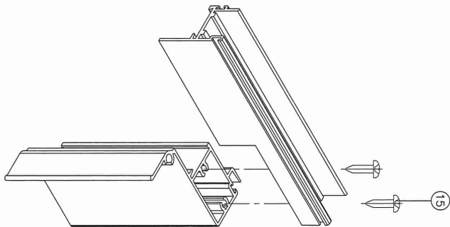
VENT TOP/BOTTOM CORNERS
