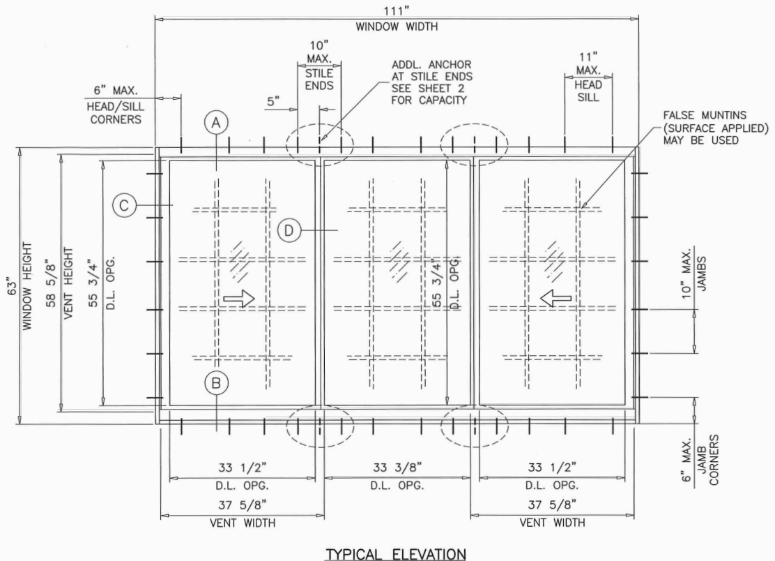
TYPICAL ELEVATION
