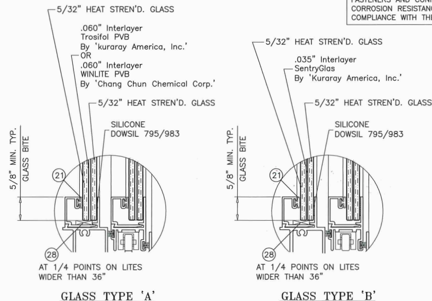
GLASS TYPE 'A'
