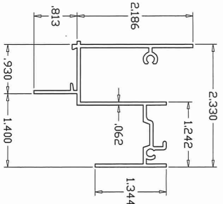
7 VENT TOP/BOTTOM RAIL
