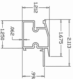
5 FIXED RAIL AT SPRING LATCHES
