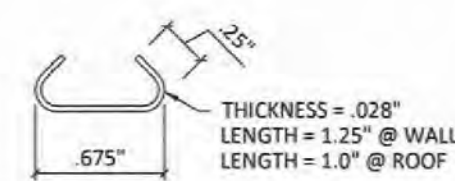
5 PANEL SKIN CLIP FULL SCALE UNGALVANIZED STEEL
