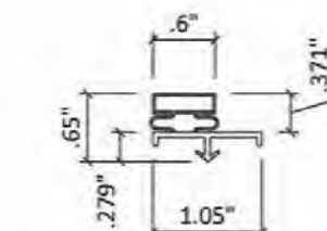
D10 DOOR GASKET HALF SCALE FLEXIBLE PVC
