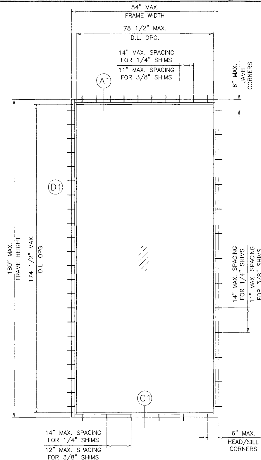
TYPICAL ELEVATION SINGLE (O) PANEL (STAND ALONE)
