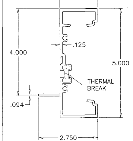
E04M VERTICAL MULLION
