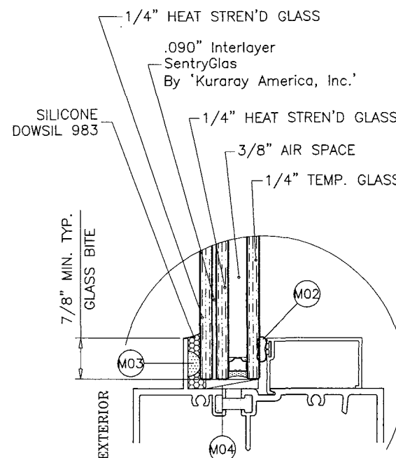
GLASS TYPE 'GL2' 1-3/16" OVERALL INSUL. LAM. GLASS
