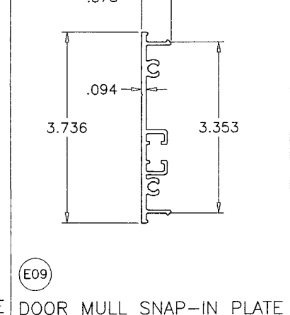
E09 DOOR MULL SNAP-IN PLATE
