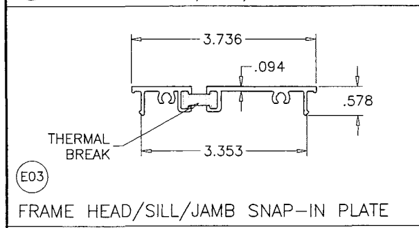
E03 FRAME HEAD/SILL/JAMB SNAP-IN PLATE
