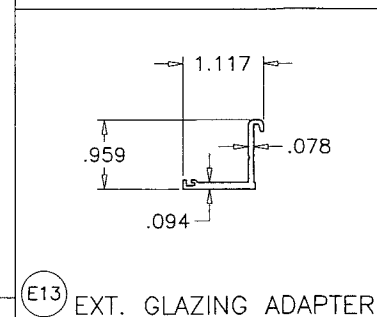
E13 EXT. GLAZING ADAPTER
