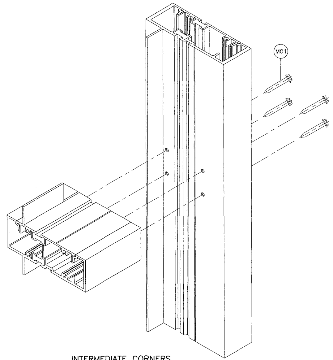
INTERMEDIATE CORNERS
