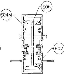
MULLION 'M2'
