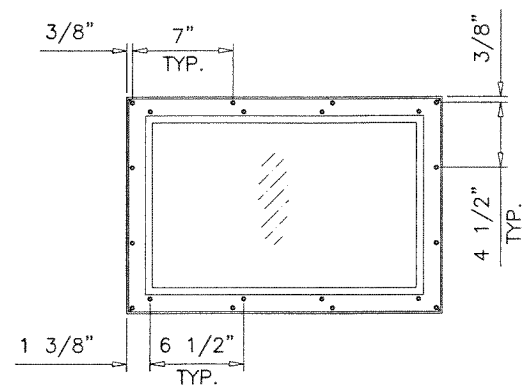
WINDOW INTERIOR ELEVATION FASTENERS SPACING
