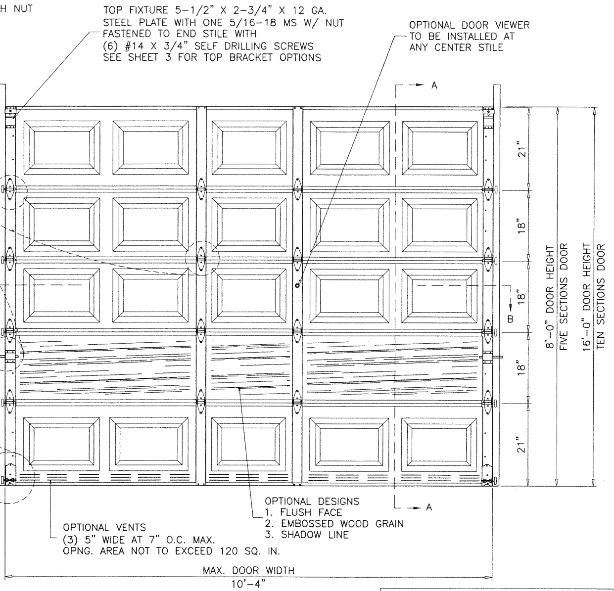
INSIDE ELEVATION RAISED PANEL EMBOSSED DOOR
