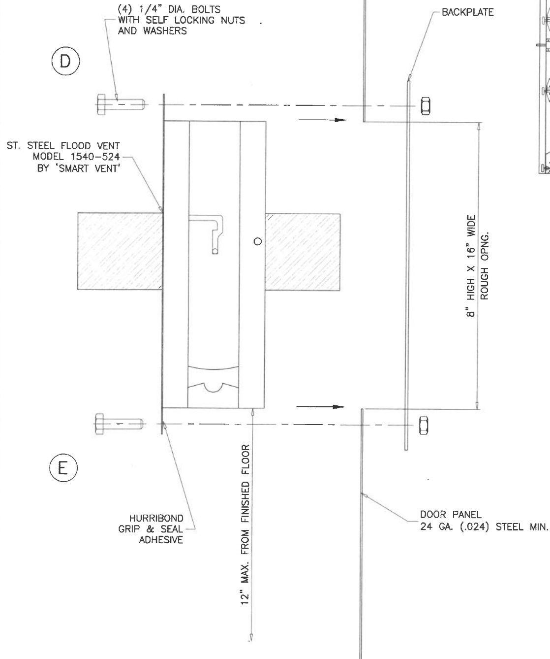
FLOOD VENT DETAIL AUTOMATIC NON-POWERED ACTIVATION & OPERATION
