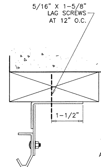
CONTINUOUS ANGLE TRACK TO WOOD BUCK
