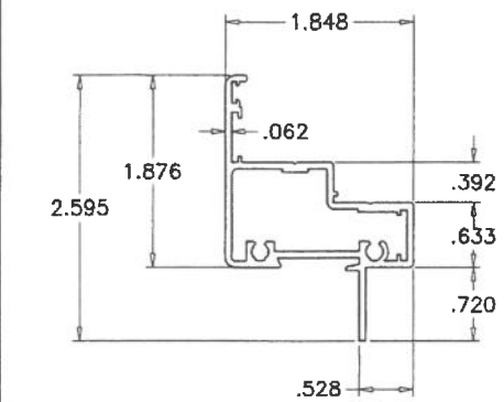
(E2) VENT
