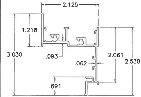
(E1) FRAME
