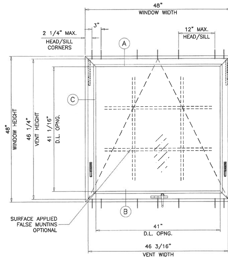
TYPICAL ELEVATION
