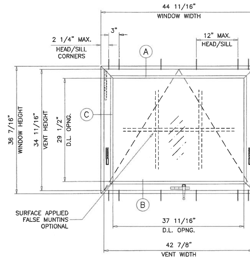
TYPICAL ELEVATION
