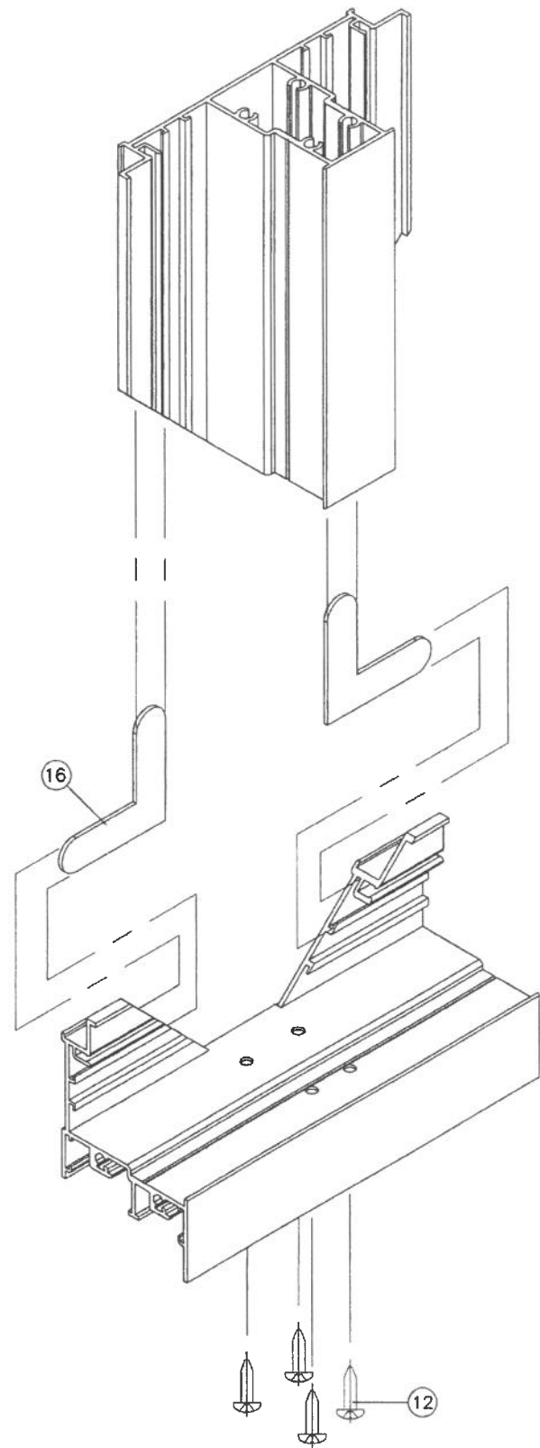
IMPOST CORNER
