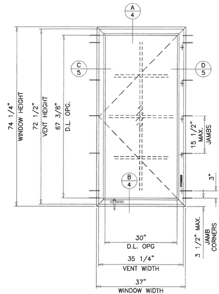
SINGLE (X)
