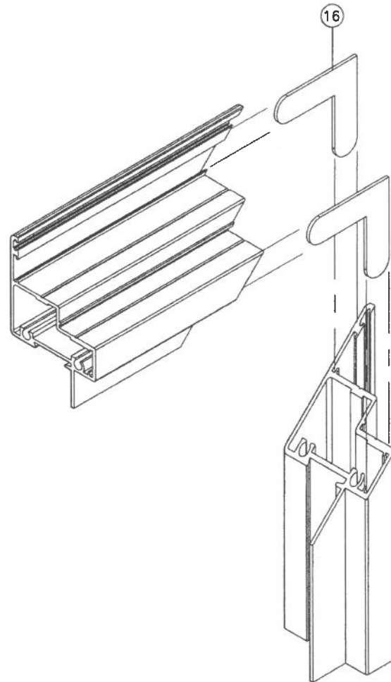
VENT CORNER
