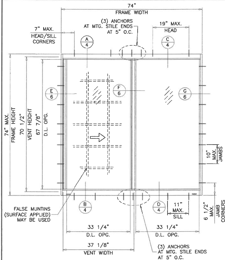
TYPICAL ELEVATION FLANGE FRAMES
