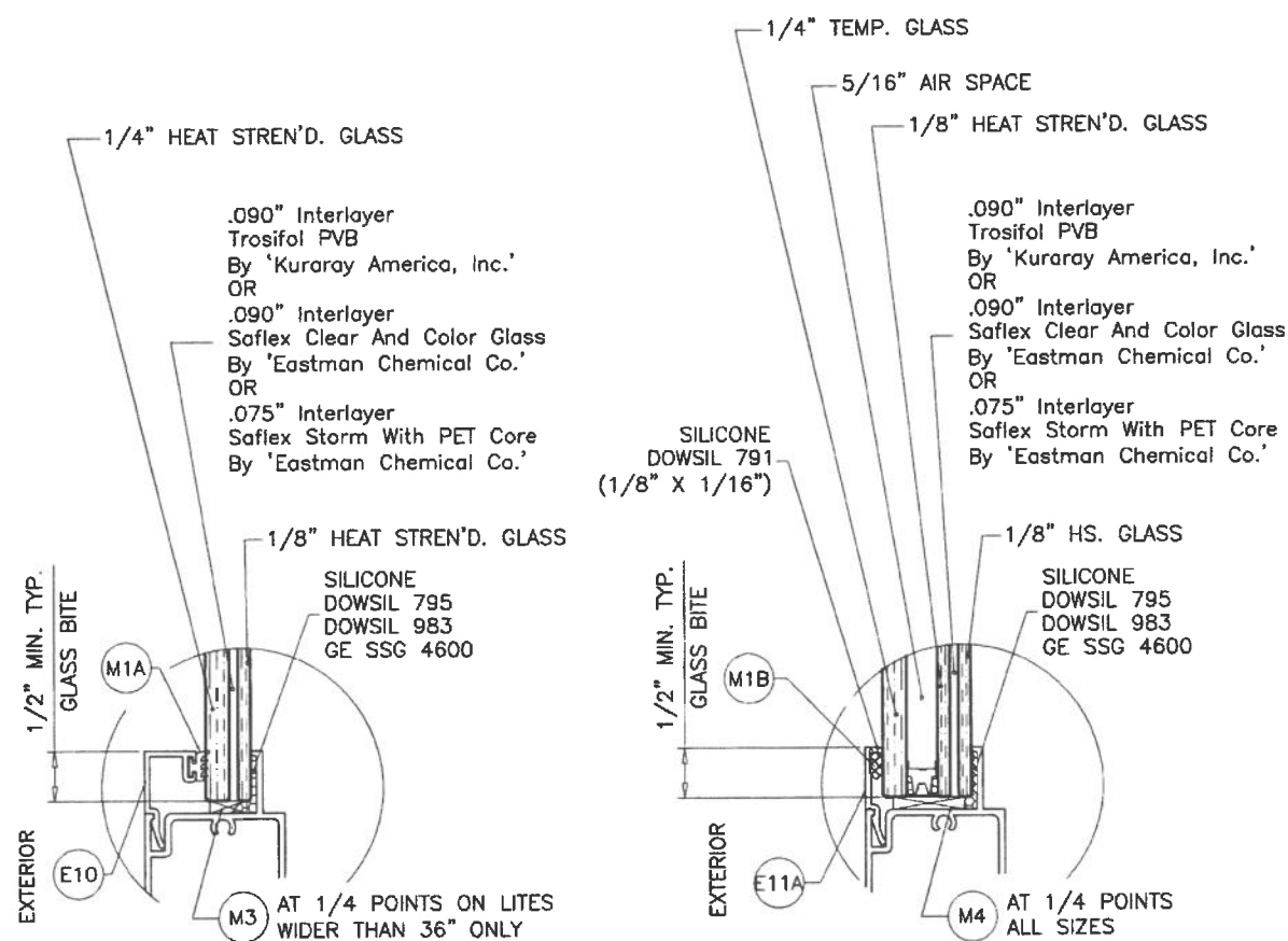
GLASS TYPE '5' 7/16" OVERALL LAM. GLASS
