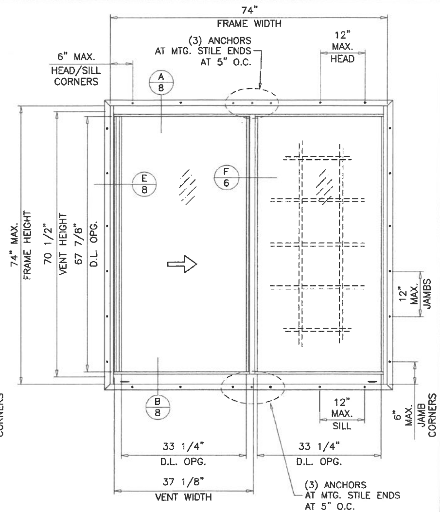
TYPICAL ELEVATION FLANGE FRAMES WITH FIN ADAPTER
