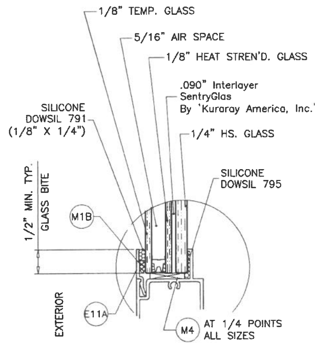
GLASS TYPE '2Ai' 7/8" OVERALL INSUL. LAM. GLASS
