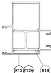
ASTRAGAL WITH REINF.
