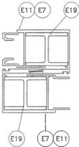
INTERLOCKS WITH REINF.
