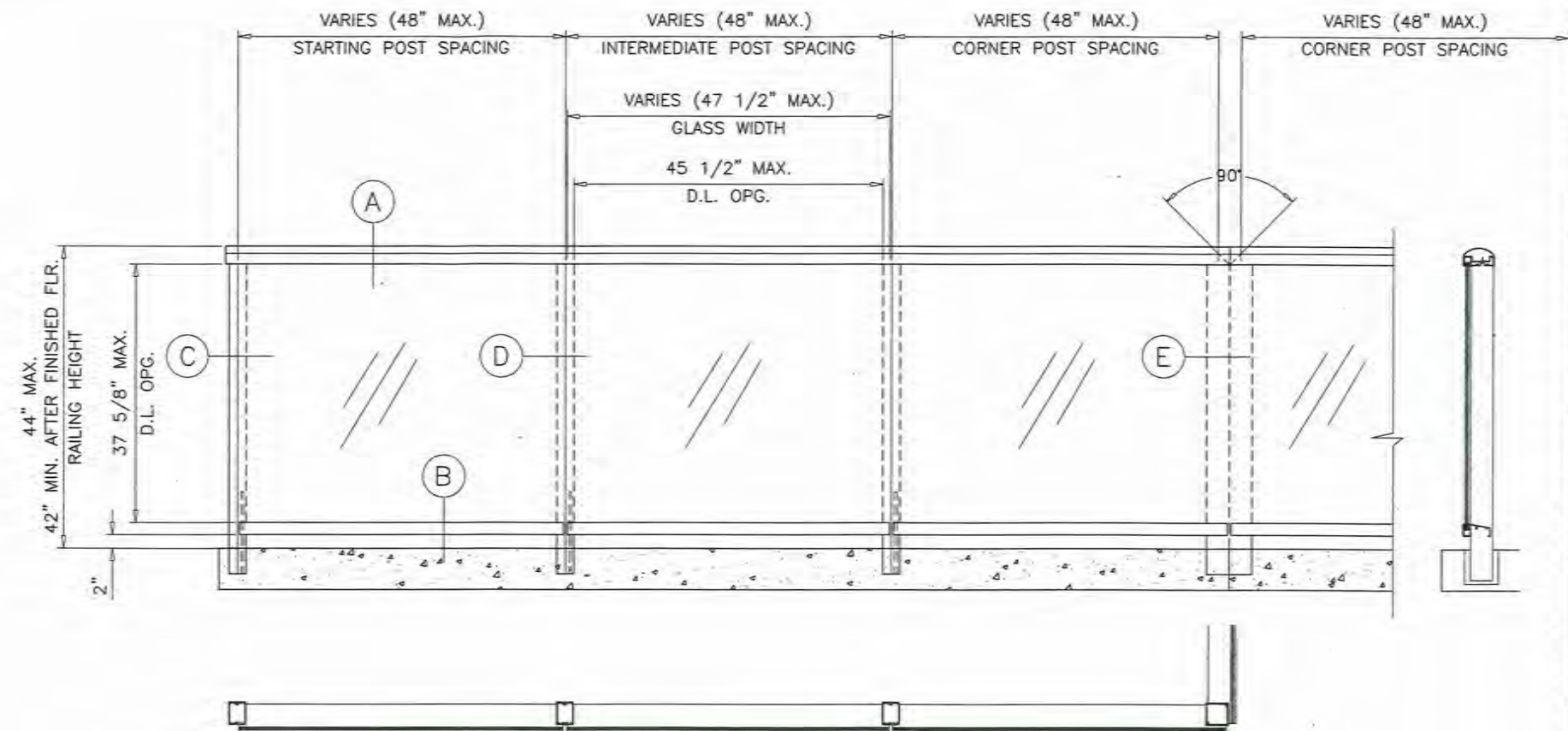
TYPICAL ELEVATION
