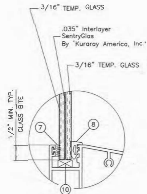
GLASS DETAIL 7/16" OVERALL LAM. GLASS
