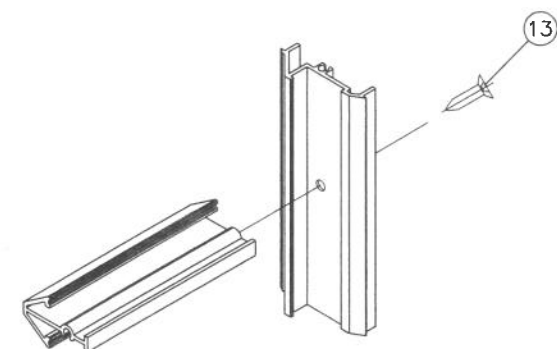
MUNTIN CORNER
