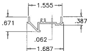
GLAZING INSERT
