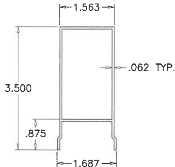
DOOR LEAF HEAD & SILL
