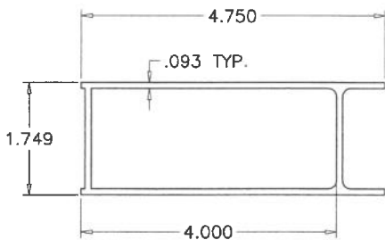
DOOR LEAF STILE
