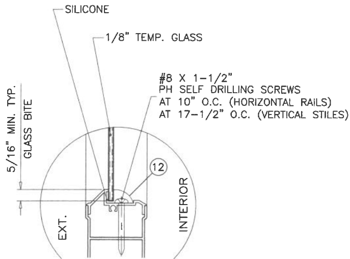
GLAZING DETAIL
