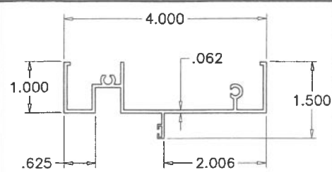
FRAME HEAD
