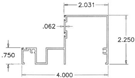
FRAME SILL
