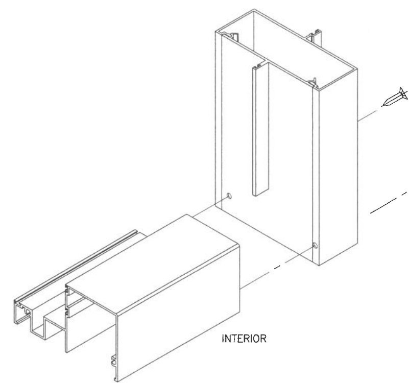
SIDELITE BOTTOM CORNER
