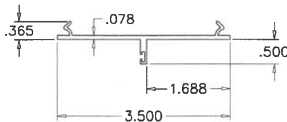
POCKET FILLER
