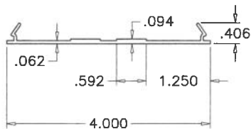
HEAD/SILL ANCHOR PLATE
