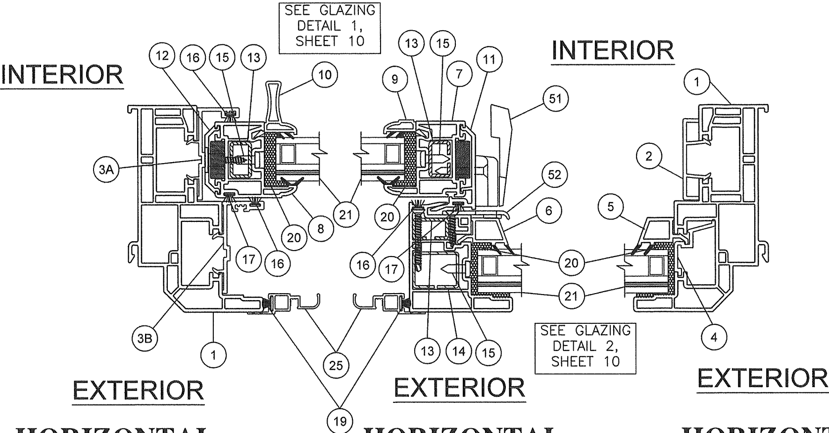
C HORIZONTAL SECTION OPERABLE LITE JAMBS - COMPONENT ID
