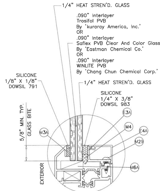
GLASS TYPE 'A1' 9/16" OVERALL NOM. THK.
