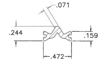
M9 12MM OFFSET
