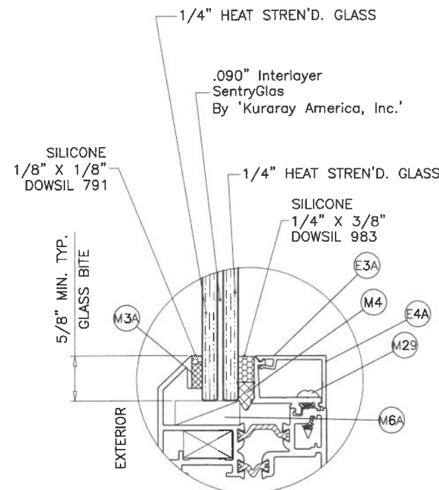
GLASS TYPE 'B1' 9/16" OVERALL NOM. THK.
