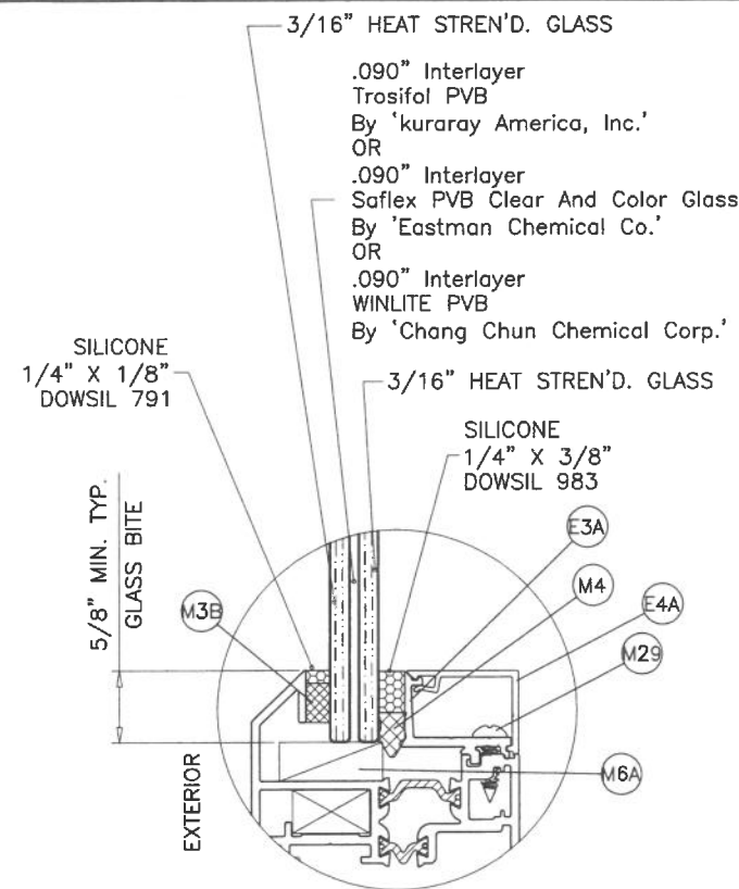
GLASS TYPE 'A' 7/16" OVERALL NOM. THK.
