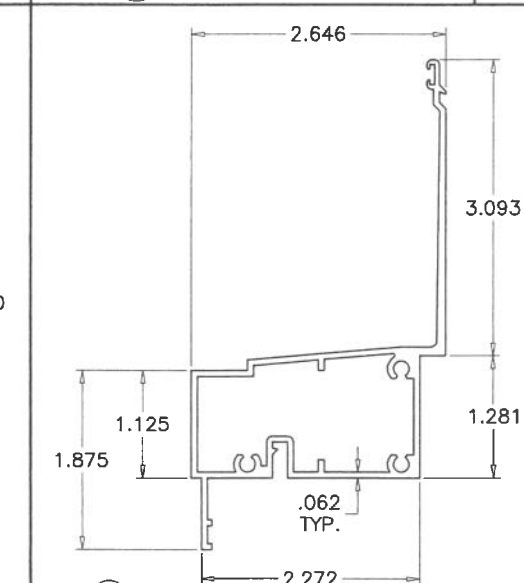
9 SILL MTG. RAIL W/ FIXED BOTTOM
