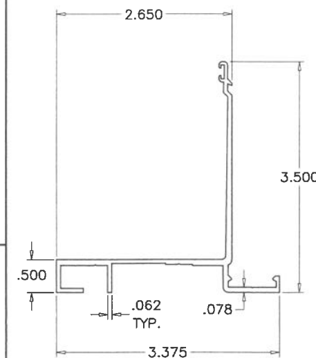
2 FRAME SILL
