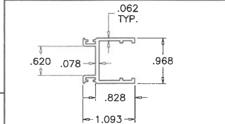
8 VENT SIDE RAIL
