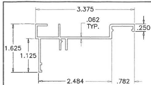
1 FRAME HEAD/SILL
