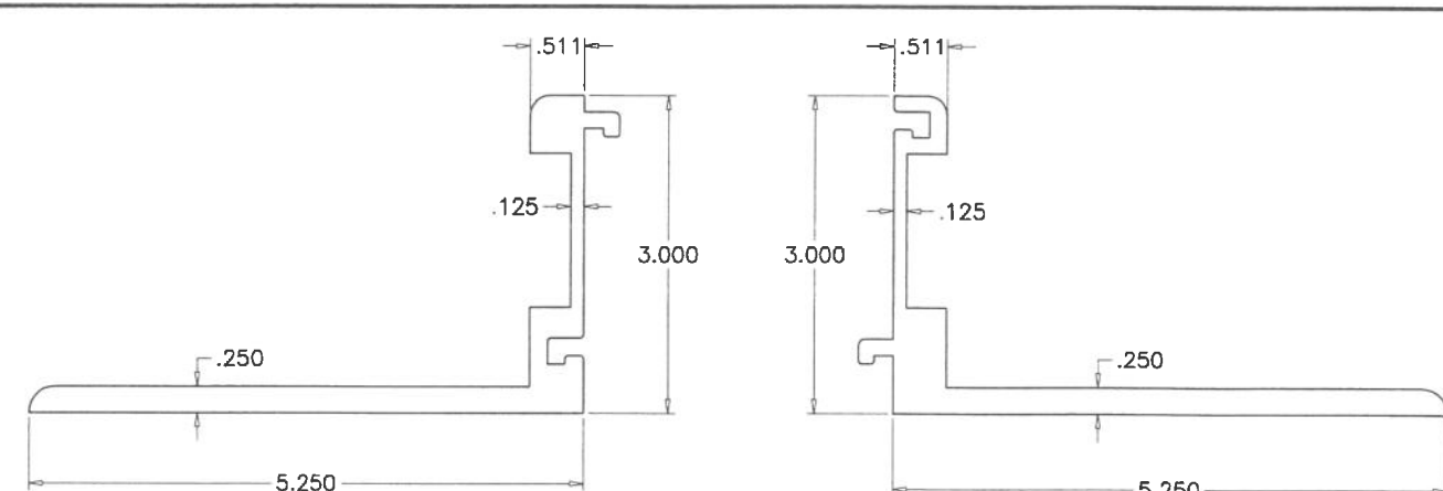
14A FEMALE ANCHOR CLIP
