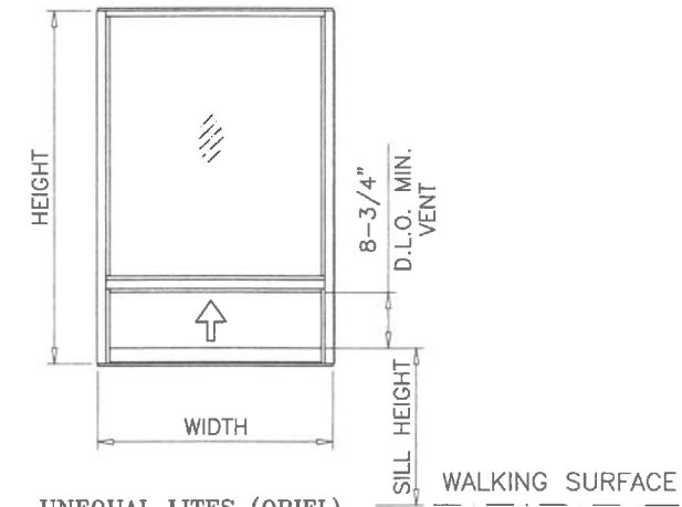
UNEQUAL LITES (ORIEL) SINGLE HUNG WINDOWS (GLASS TYPE D)
