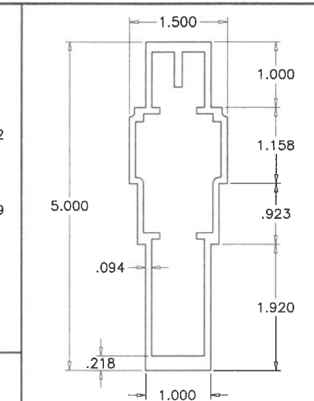
11 STD. MULLION
