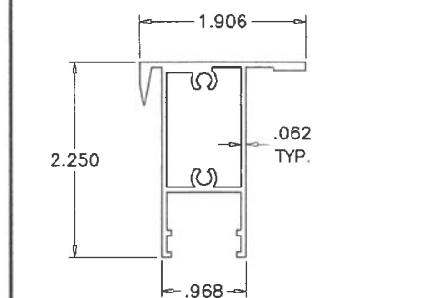
4 VENT TOP RAIL
