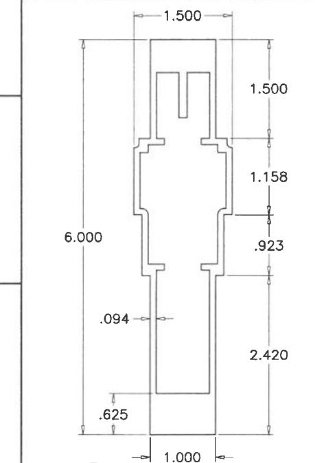
11A H.D. MULLION
