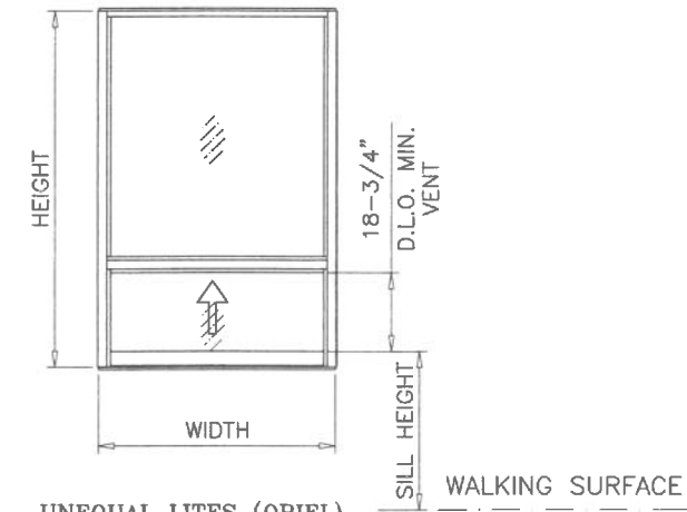
UNEQUAL LITES (ORIEL) SINGLE HUNG WINDOWS (GLASS TYPES A, B & C)
