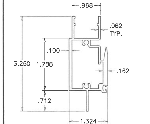
3 MEETING RAIL
