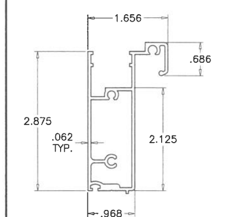
6 VENT BOTTOM RAIL
