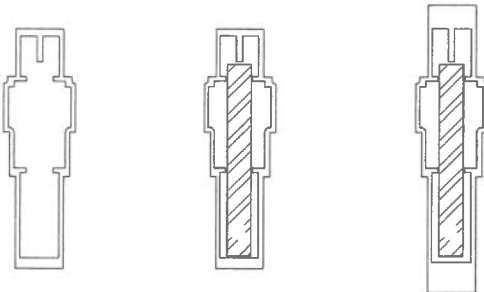
STD. MULLION UNREINFORCED STD. MULLION REINFORCED H.D. MULLION REINFORCED
