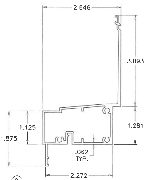
SILL MTG. RAIL W/ FIXED BOTTOM
