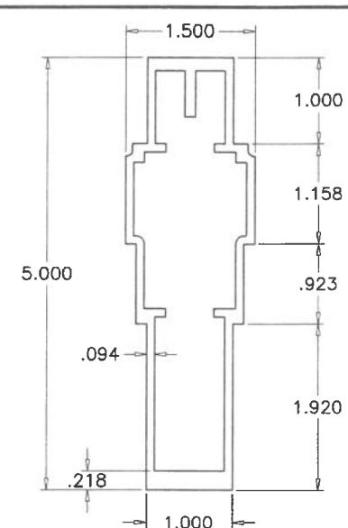
11 STD. MULLION
