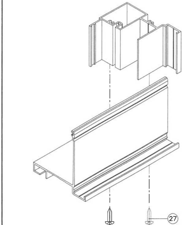
FRAME CORNERS DETAIL
