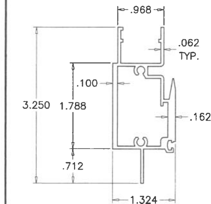
3 MEETING RAIL
