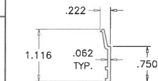
12 VENT LATCH
