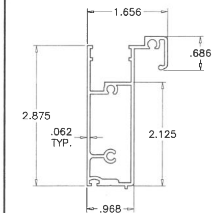
6 VENT BOTTOM RAIL
