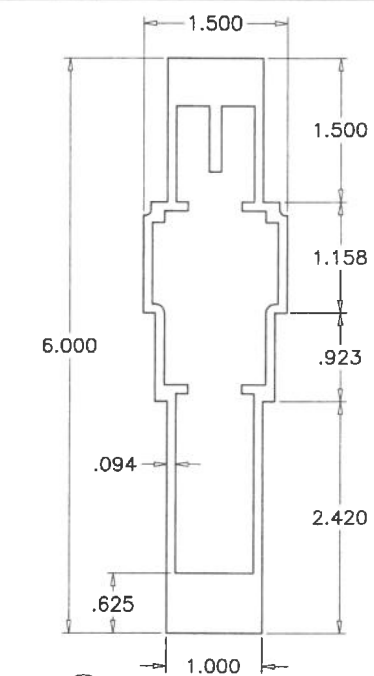
11A H.D. MULLION
