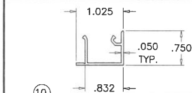
INSTALLATION TRACK COVER
