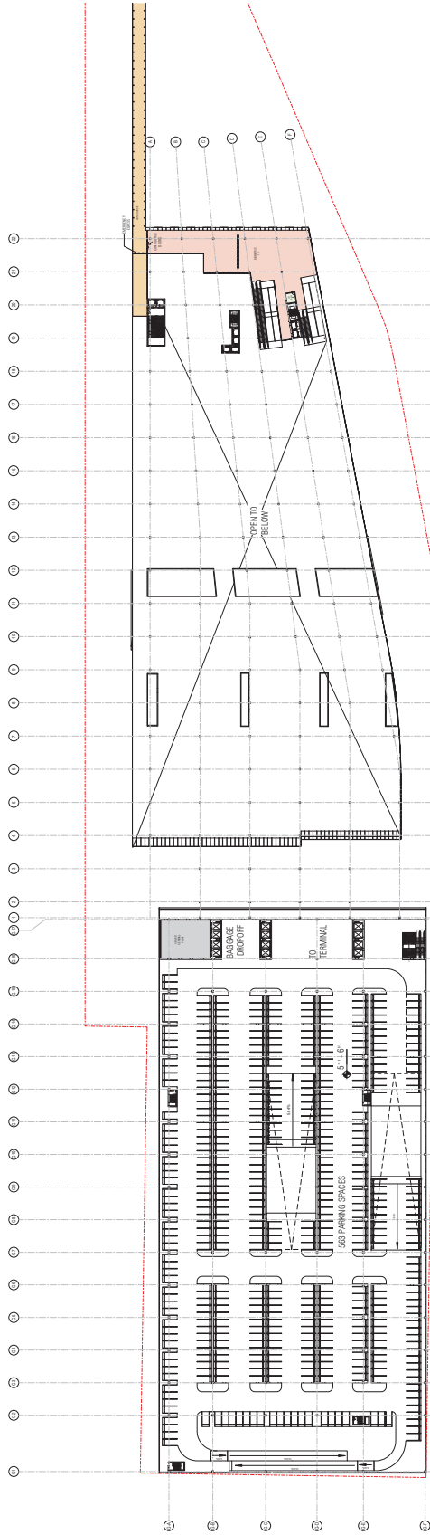
2ND LEVEL MEZZANINE PT. 1 1/8" = 1'-0"
