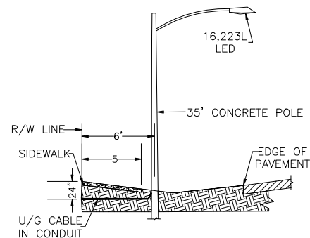
TYPICAL UNDERGROUND INSTALLATION N.T.S.
