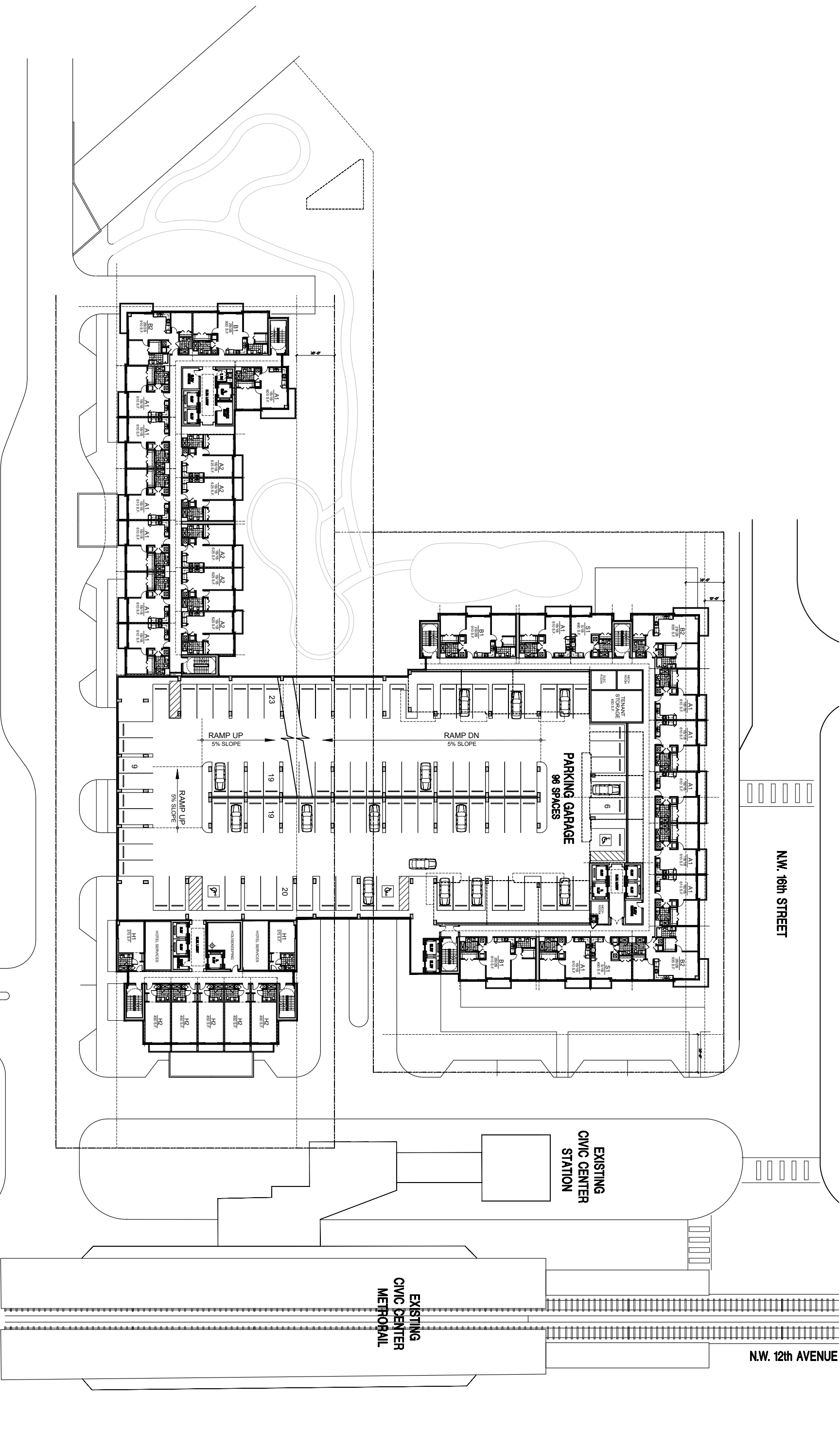
TYPICAL GARAGE LEVELS LEVELS: 2-9 SCALE: 1/8" = 1'-0"
