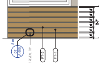
03 Typical Reveal Detail SCALE: 3/4" = 1'-0"
