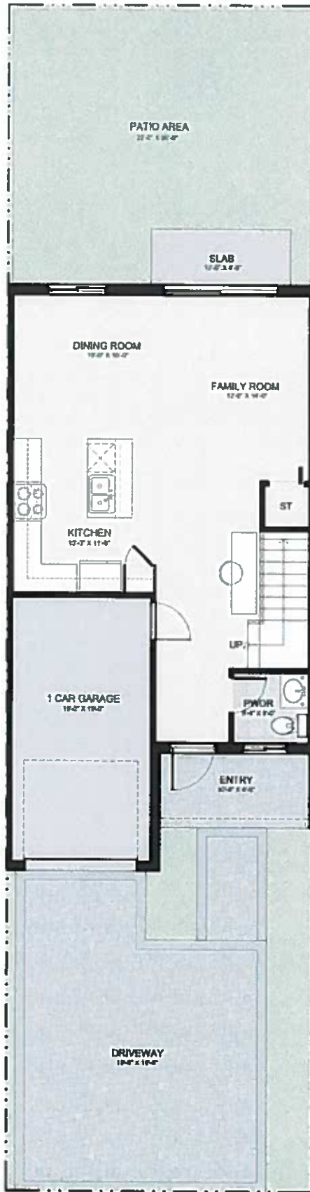
FIRST FLOOR
