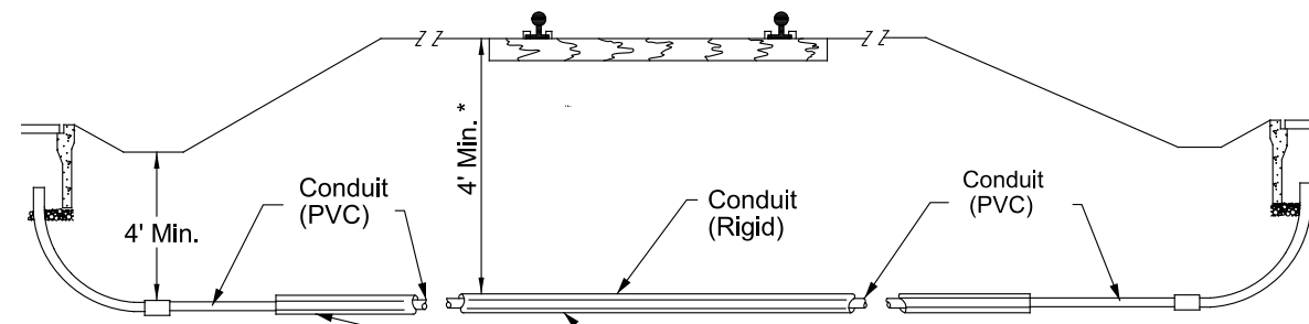
FIGURE I FOR USE UNDER RAILROADS
